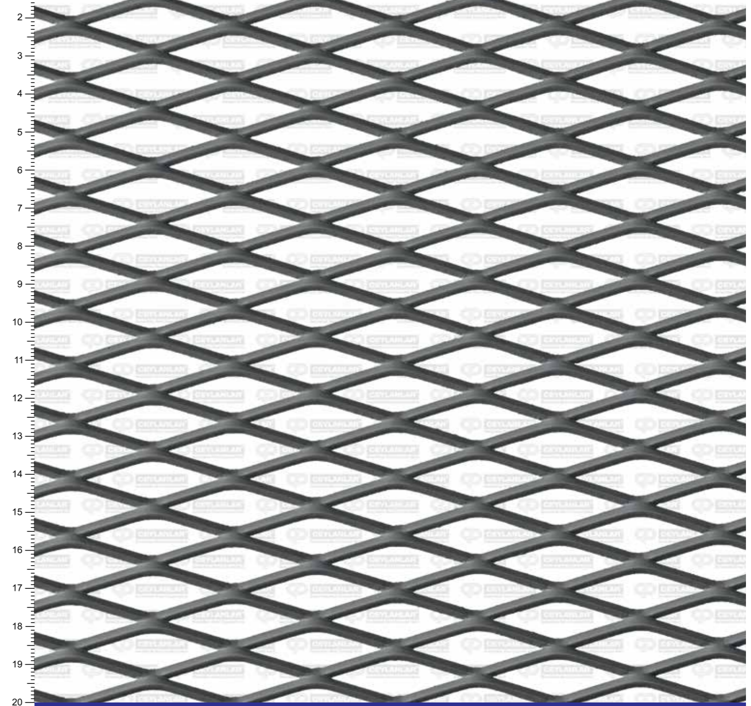
D42-3 - 14 x 42 x 2 x 3 mm
