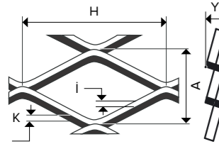
New York 115-15 - 50 x 115 x 2 x 15 mm
