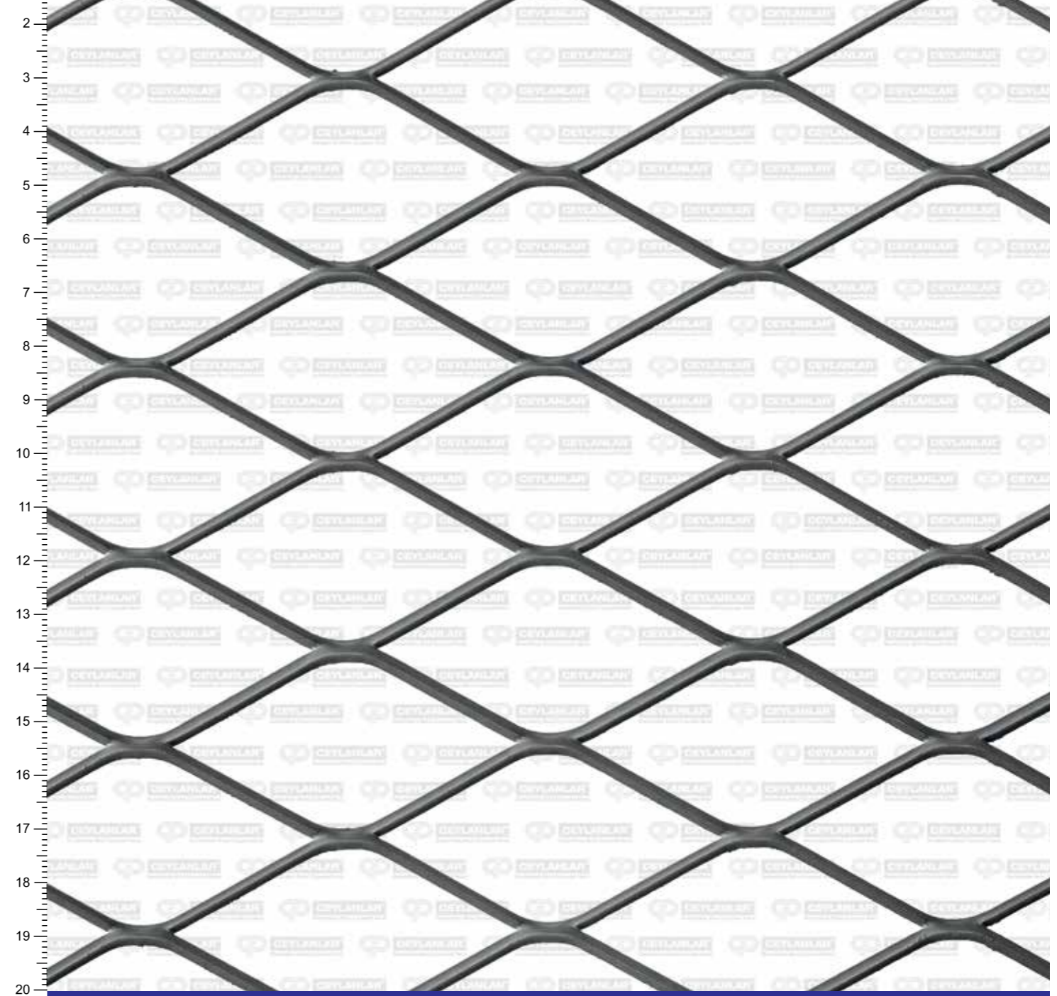
D75 - 35 x 75 x 2 x 3 mm
