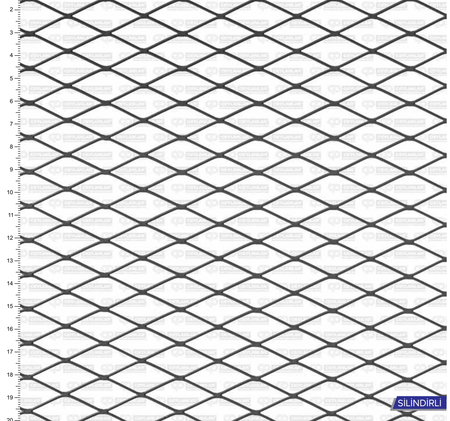
DF32 - 13.5 x 32 x 0.5 x 0.95 mm
