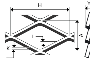
DF50 - 20(23) x 50 x 2 x 3.25 mm
