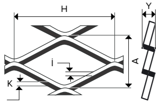
Moscow 30 - 12 x 30 x 2 x 3 mm
