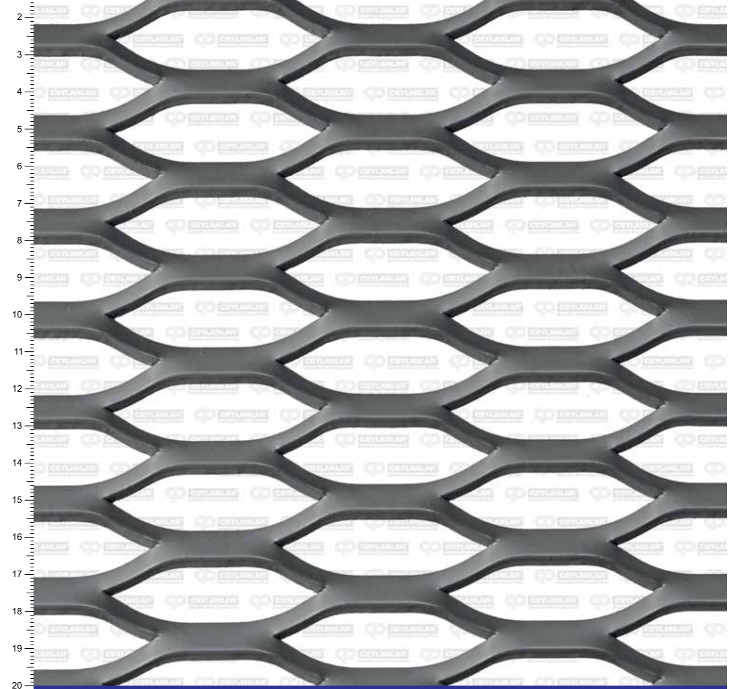
D91 - 28 x 90 x 4 x 6 mm
