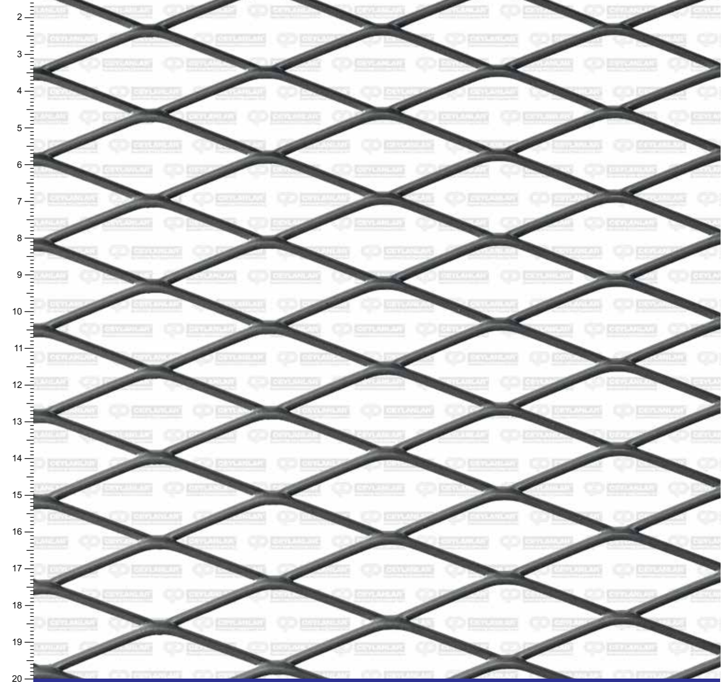
D62 - 23 x 62 x 2 x 3 mm
