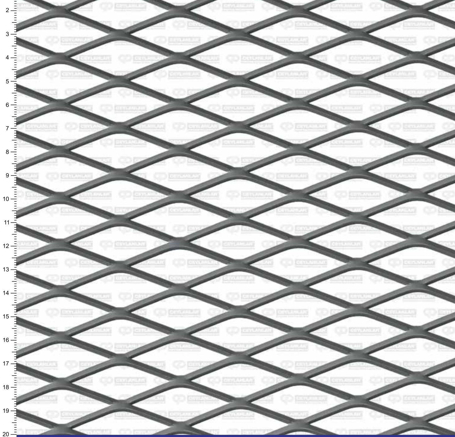
D50 - 20 x 50 x 2 x 3 mm
